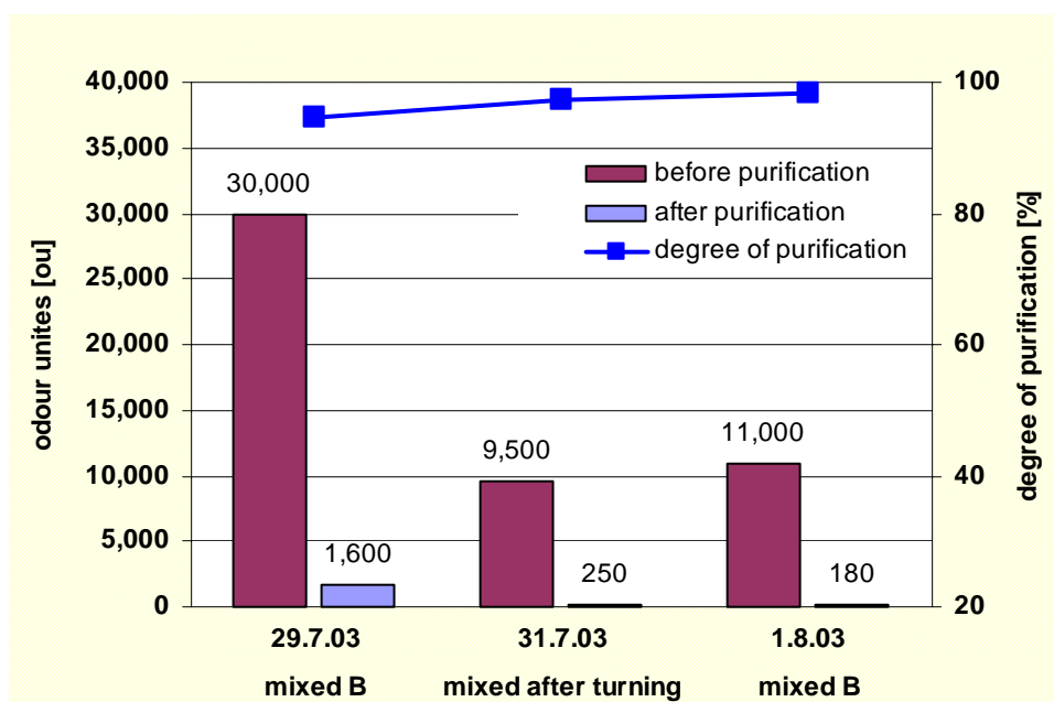
Figure 5: Odour units recorded before and after purification by biofilter (sucked air mixed from 1 and 4-5 week old material))
