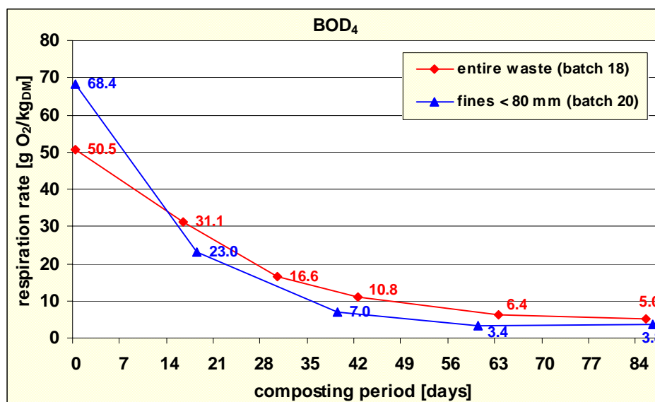
Figure 2: Change in respiration rate (using SRI, BOD 4 ) during the composting of MSW using New Earth Composting Technology.
