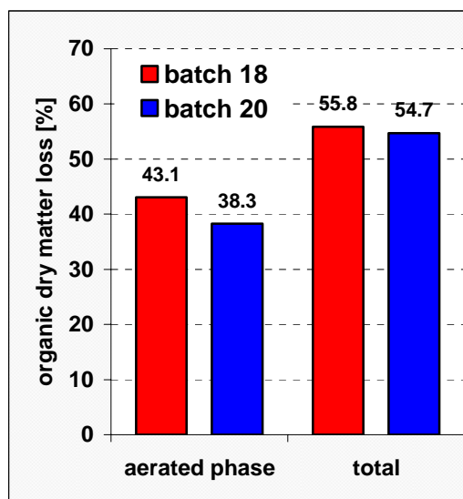
Figure 1. Loss of dry matter of MSW during the aerated phase of the composting process and for the aerated and maturation phase as a whole.
