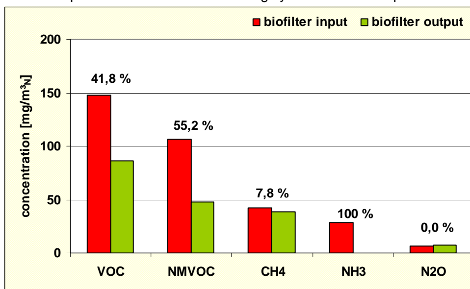
Figure 4: Concentration of different substances before and after the exhaust air treatment system; the numbers describe the level of cleaning in relation to the starting concentration
